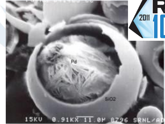
Porous wall hollow glass microspheres
